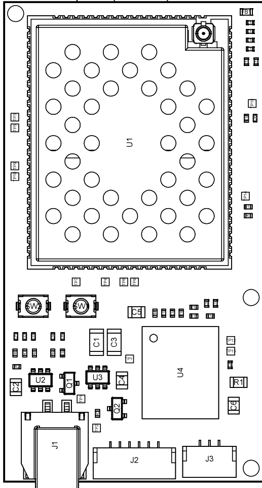
View from Top side (Scale 2:1)
