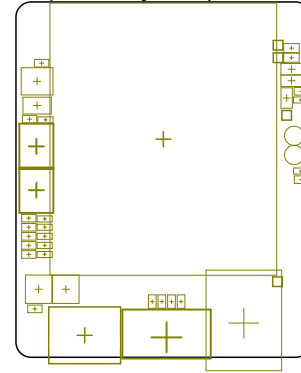
Top Courtyard (Scale 1:1)
