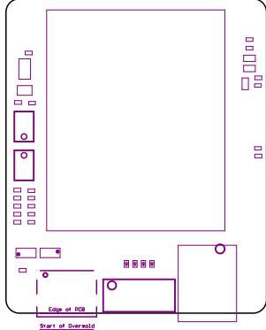
Top Assembly (Scale 1:1)
