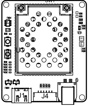
View from Top side (Scale 1:1)
