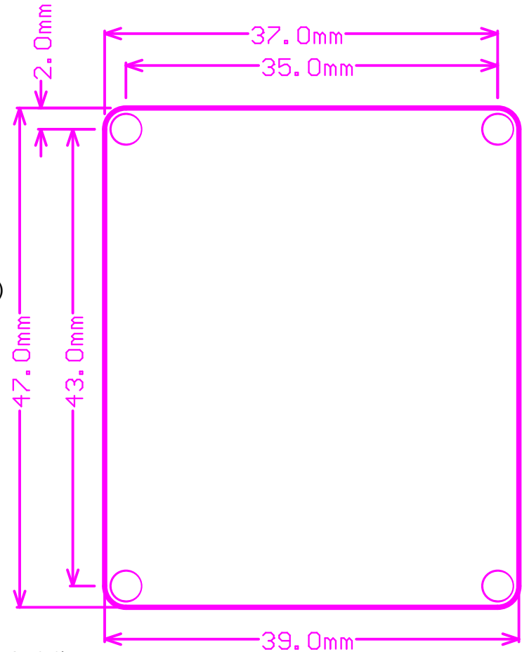
View from Left side (Scale 1:1)
