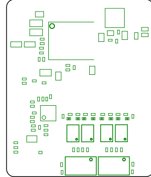
Bottom Assembly (Scale 1:1)
