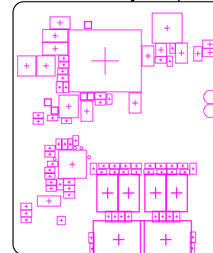
Bottom Courtyard (Scale 1:1)
